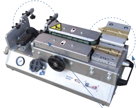
Configured machine with both inletguides and adaptor plates. Ready to operate.
